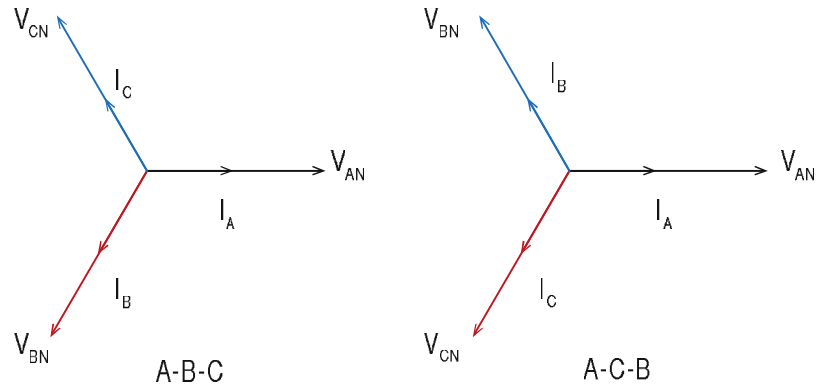
Figure 2. Vector diagram of data file and reference vector diagram for a three phase wye
